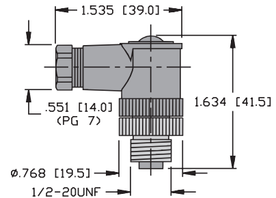
Male Connector
