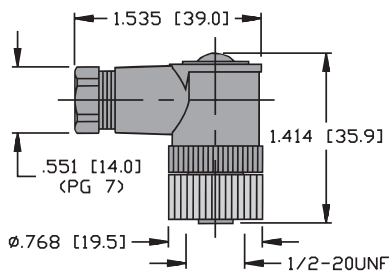
Female Connector
