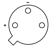
Figure 3. 3-Pin TO-52
