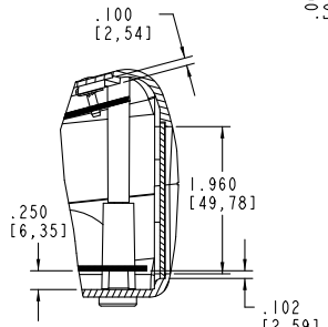
DETAIL D SCALE 1200
