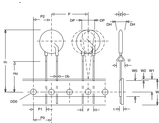
UNDER CRIMPED LEADS "ZU"
