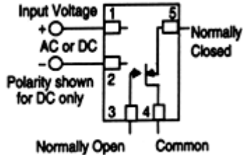
Single Pole - Double Throw
